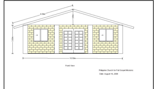
27' x 36' Proposed Structure
